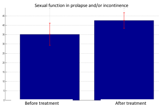
Graph 23: Statistical analysis PISQ-12
