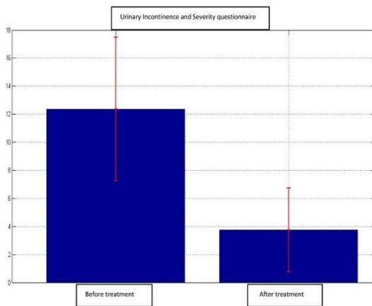
Graph 20: Statistical analysis ICIQ-SF
