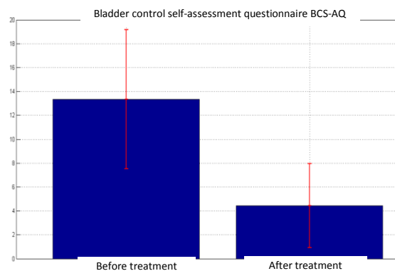
Graph 22: Statistical analysis BCSA-AQ
